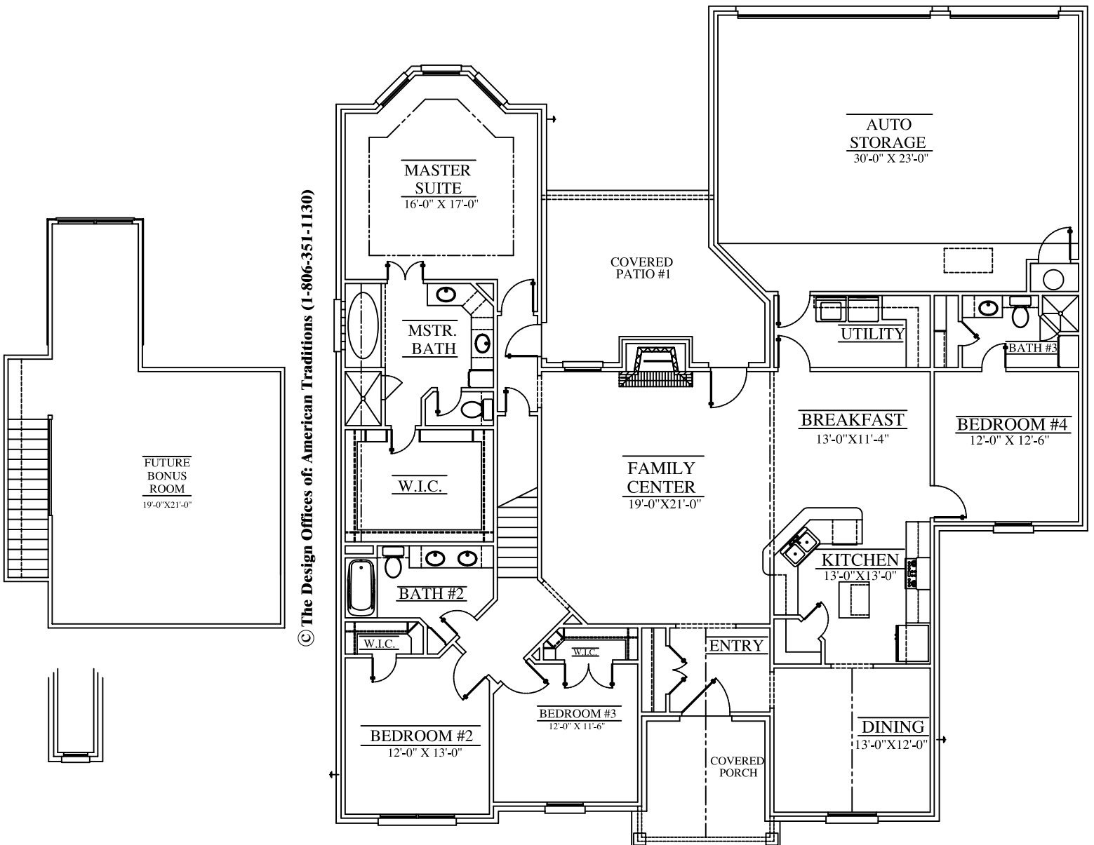
LIVING 3,100 SQ. FT. PLAN NO.01097-24
